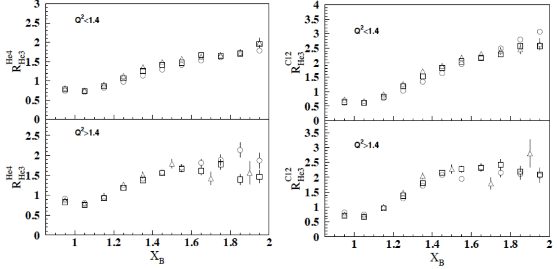
Figure 2.2: The cross section ratio per nucleon of {}^4\text{He} (left plots) and {}^{12}\text{C} (right plot) to {}^3\text{He} . The top plots show the ratio for Q^2 < 1.4 without an observation for scaling. The bottom plots show ratio for Q^2 > 1.4 with scaling in the region 1 < x_{bj} < 2 [38].
