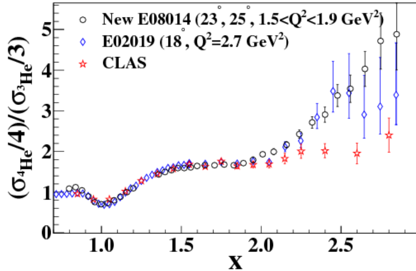
Figure 2.16: A comparison of 3 different data sets for 3N-SRCs studies from JLab's hall A, B and C. They are in good agreement in the 2N-SRCs region 1 < x_{bj} < 2 . For the 3N-SRCs region x_{bj} > 2 , the data from E08-014 (hall A) and E02-019 (hall C) agree with each other but differ from the CLAS (hall B) data [55]
