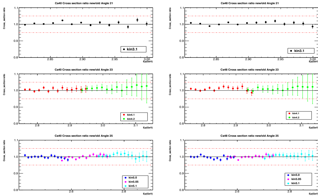
Figure 5.28: The ratio of the extracted cross using the first iterated cross section model to the extracted cross section using initial cross section model section as a function of E' for different kinematic settings. The left plots are for ^{40}\text{Ca} while the right plots are for ^{48}\text{Ca} . Two red dashed lines in each plot shows \pm 5\% variation from one.
