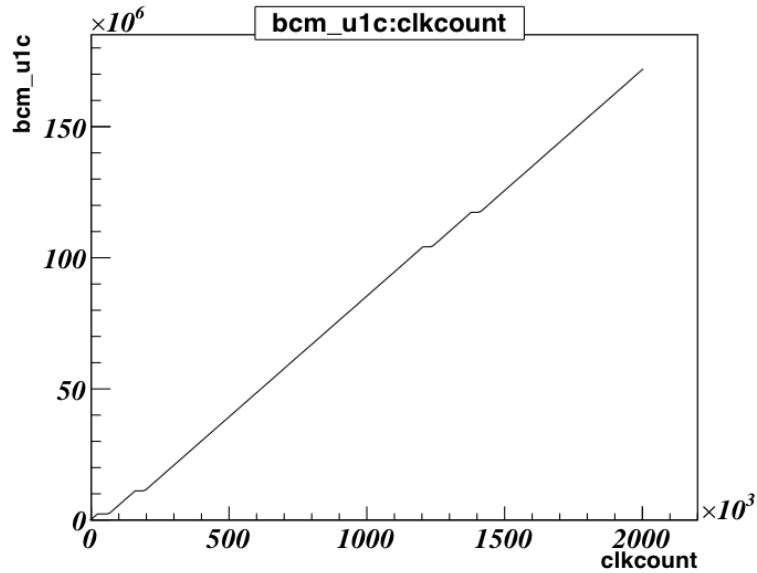
Figure 4.29: The number of BCM counts from bcm-u1 vs number of count from the clock. When beam trips, the bcm count doesn't change.
