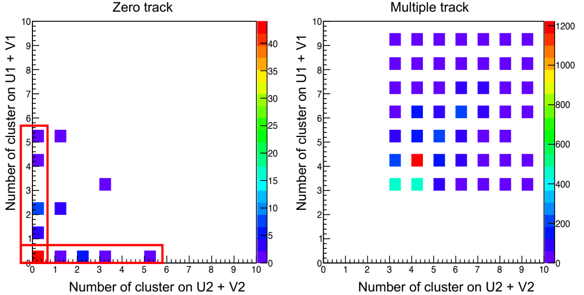
Figure 4.42: Total number of cluster from wire plane U, V for each VDC chamber. The left plot is for the Zero tracks, showing that at least one of wire planes has no clusters. The right plot is for Multiple tracks, showing that at least one of wire planes have more than one cluster.
