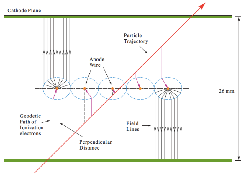
Figure 4.40: A cluster with 5 cells in a wire plane in the VDCs [65, 79].
