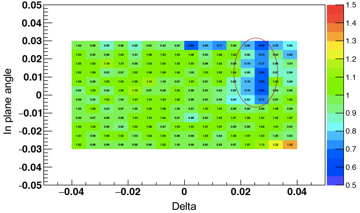
Figure 5.4: The 2D Yield ratio as function of in plane angle \phi_{tg} (rad) vs relative momentum dp shows a specific region where the yield ratio drops. This occurs at dp \sim 0.03 and \phi_{tg} > -0.005 .
