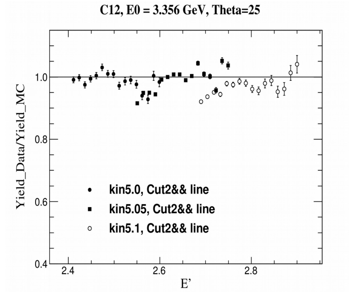
Figure 5.1: Data/MC Yield ratio for 3 different overlap kinematics binned in E'
