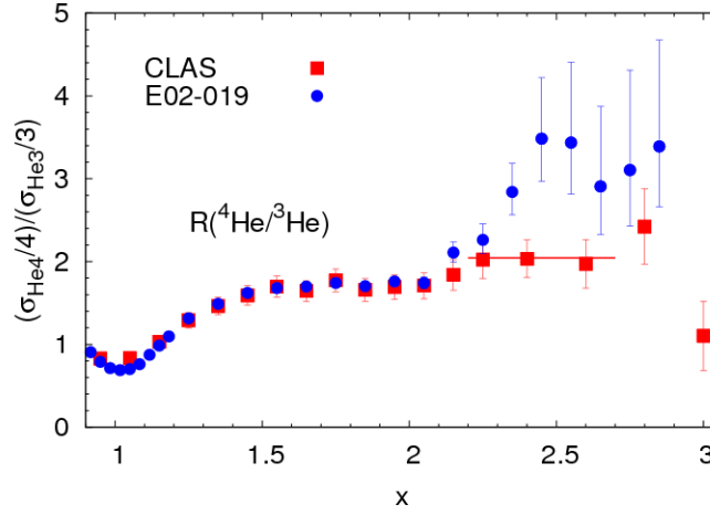
Figure 2.5: The comparison of the cross section ratio R(^4\text{He}/^3\text{He}) per nucleon between CLAS [39] data and E02-019 data [42].
