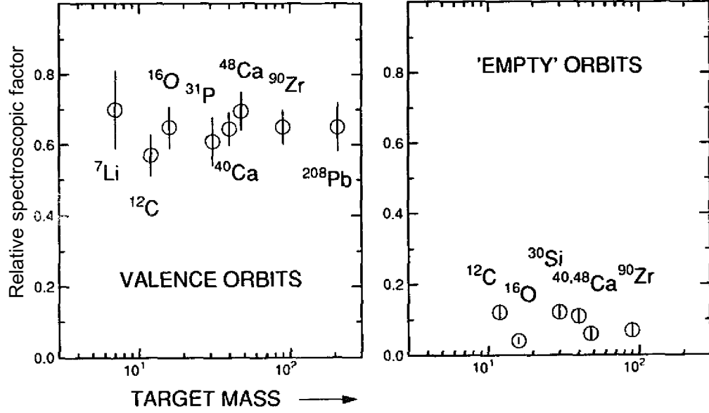
Figure 1.7: Left plot shows the spectroscopic factor for valence shell from A(e, e'p) experiment at NIKHEF as a function of target mass. For nuclei A > 7 this spectroscopic factor is almost a constant \sim 65\% . Right plot shows a small spectroscopic factor for the shell above but close to valence shell [7].
