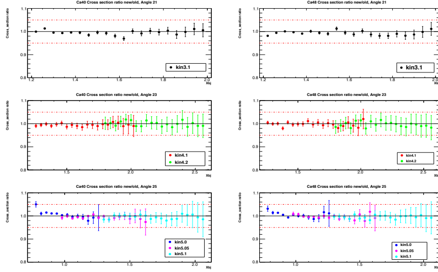
Figure 5.29: The ratio of the extracted cross using the first iterated cross section model to the extracted cross section using initial cross section model section as a function of x_{bj} for different kinematic settings. The left plots are for ^{40}\text{Ca} while the right plots are for ^{48}\text{Ca} . Two red dashed lines in each plot shows \pm 5\% variation from one.
