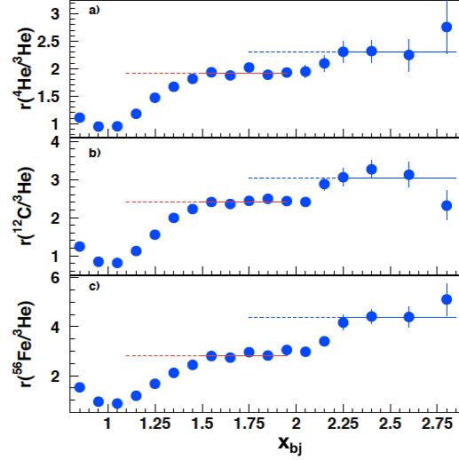
Figure 2.3: The ratio of cross section from different nuclei to {}^3\text{He} shows 2 scaling regions. The scaling in the range of 1 < x_{bj} < 2 was claimed as results of 2N SRCs, while second scaling x_{bj} > 2 was assumed to be the indication of 3N SRCs [39].
