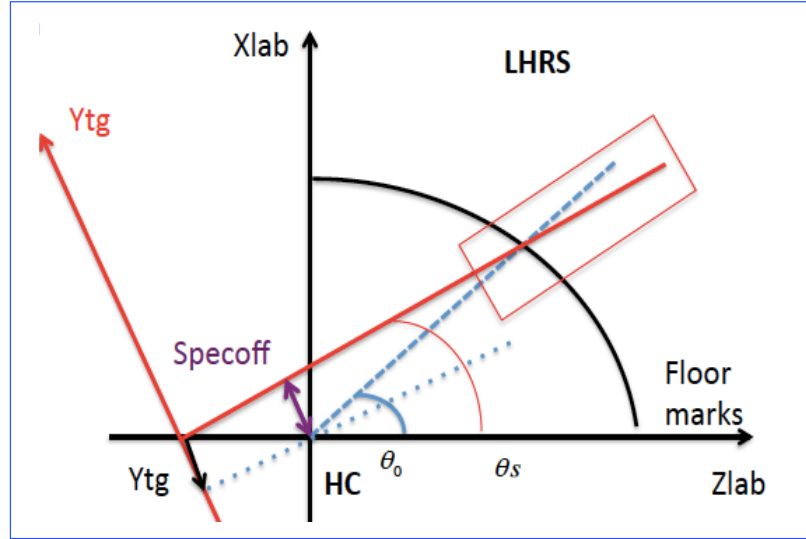
Figure 4.46: The convention for mis-pointing study in the Lab and the target coordinator system.
