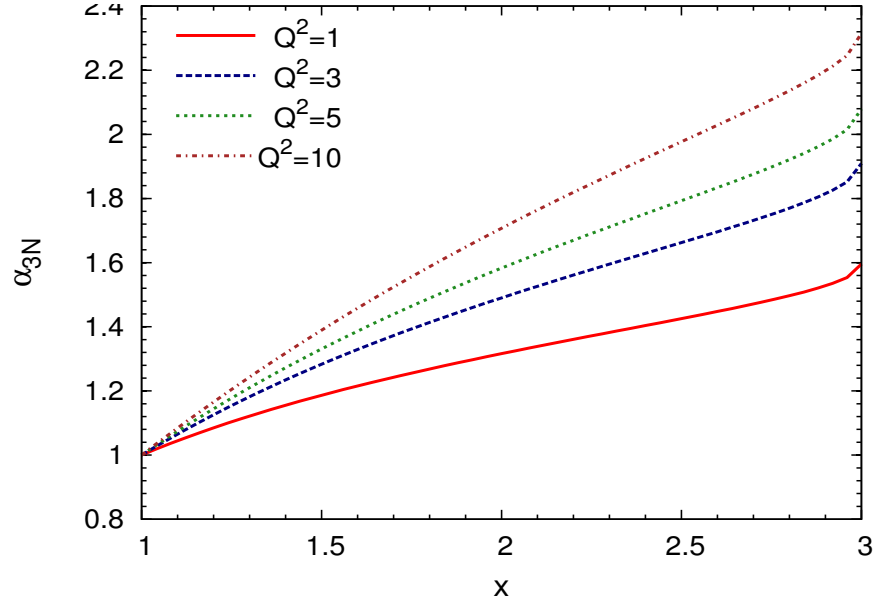
Figure 1.17: The 3N SRCs kinematic calculation as a function of x_{bj} and \alpha_{3N} , a function of x_{bj} and Q^2 [35].
