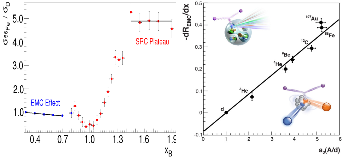
Figure 2.15: A quantitative comparison of the EMC strength and SRC scaling factors for different nuclei. The left plot shows the cross section ratio per nucleon for Fe to ^2\text{D} as function of x_{bj} . The EMC effect and SRC scaling both is visible. The right plot shows the correlation between the EMC strength and the SRC scaling over a range of nuclei.
