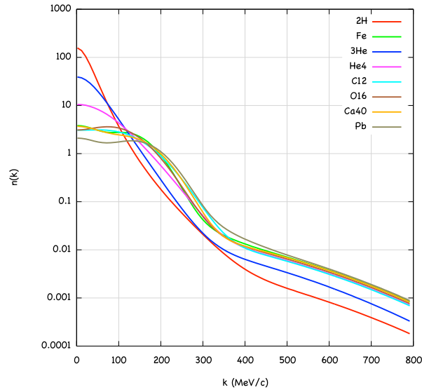
Figure 1.11: The momentum distribution for different nuclei, scaled from the ^2\text{D} momentum distribution using different scaling factors [21].
