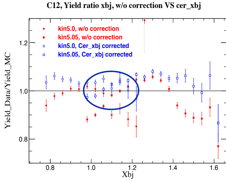
Figure 5.12: The red points are the yield ratio as function of x_{bj} for two overlap kinematic settings, Kin5.0 and Kin5.05, before the local efficiency correction, and the blue points are the results after the correction.
