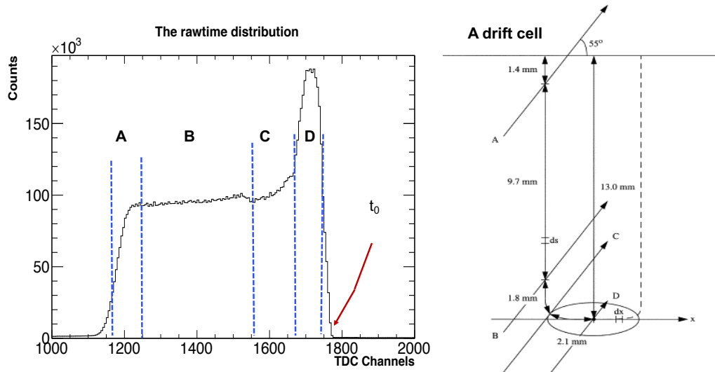
Figure 4.11: Left plot: the VDCs raw-time distribution as a function of TDC channels. Right plot: A drift cell for a wire with 4 different trajectories crossing the cell.
