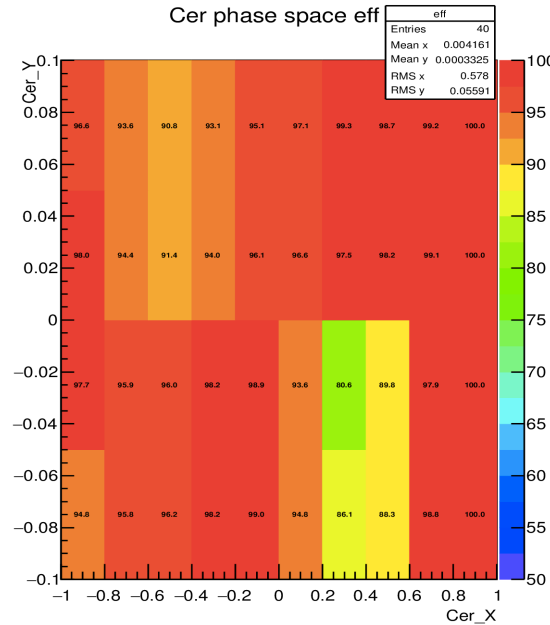
Figure 5.8: The plot shows the local efficiency as function of Cherenkov position.
