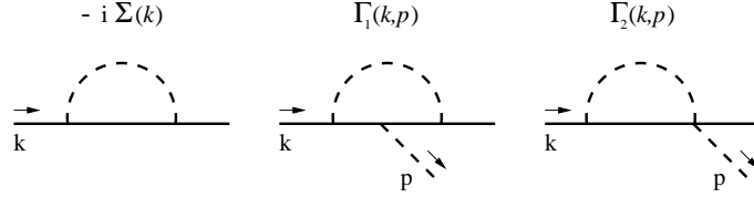
Figure 6.3. One-loop self-energy, and vertex corrections.
