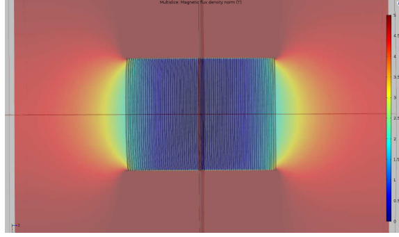
Figure 5: A shielding magnet used to zero out an external field of 1.7 T with a slight field gradient using COMSOL Multiphysics Simulation Software.
